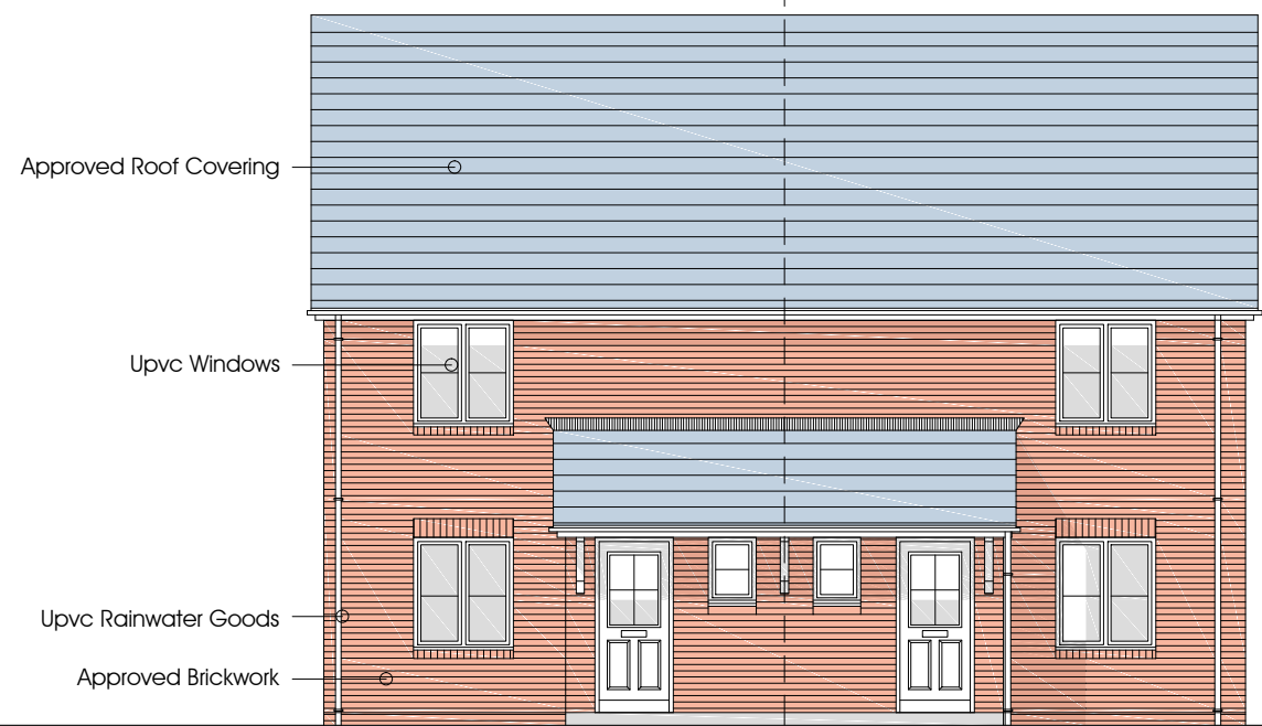
entrance entrance front & rear elevation
